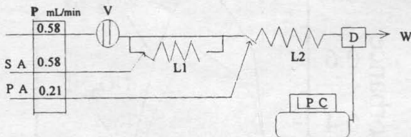
FIGURE 2 Schematic diagram of FI manifold employed for the simultaneous determination of nitrite and nitrate: P, pump; V, valve; L(1, 2), reaction coil; D, detector; W, waste; PC, personal computer; SA, sulfanilic acid; PA, N-phenylanthranilic acid
