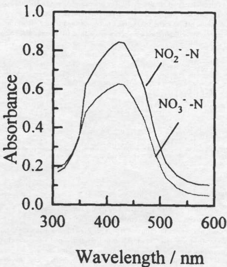
FIGURE 1 Absorption spectra of N-phenylanthranilic acid in the presence of 0.6 \mu\text{g ml}^{-1} of nitrite and 0.8 \mu\text{g ml}^{-1} nitrate, pH= 0.5
