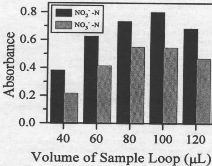
FIGURE 4 Effect of sample size on the sensitivity: nitrite, 0.6 \mu\text{g ml}^{-1} ; nitrate, 0.8 \mu\text{g ml}^{-1} pH= 0.5
