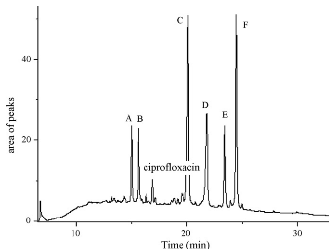
Fig. 6. HPLC chromatogram of the photocatalytic degradation of ciprofloxacin for 40 min. Peaks A to F: degradation compounds.
