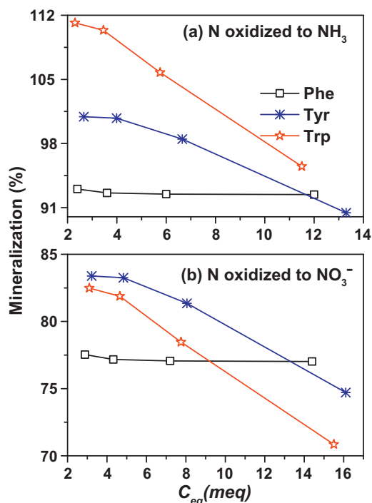
Fig. 3. Photoelectrocatalytic degradation of Phe, Tyr and Trp. (a) Mineralization percentage against C_{eq} for N oxidized to NH_3 and (b) to NO_3^- .
